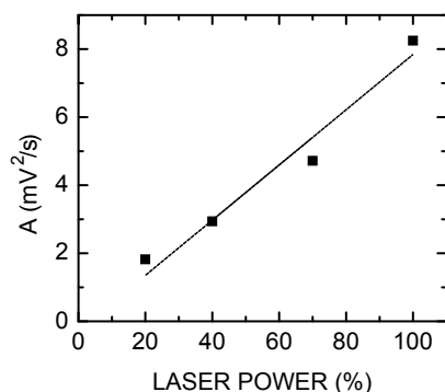
FIGURE 9 Area under the spectral density, obtained by a fit of the measured curve to a Lorentzian, as a function of laser power (100% corresponds to 1 W at the laser).
