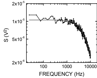
FIGURE 7 Brownian motion of a captured bead. Power spectral density of the interferometer signal U_\omega for a glass bead of 1 \mu\text{m} in diameter. The bead is captured in water with a laser power of 700 mW (70% of our maximum laser power). The fit to a Lorentzian gives two parameters: the cutoff frequency f_c (here 5.7 kHz) and the area under the curve (here 4.72 \text{mV}^2/\text{s} ).
